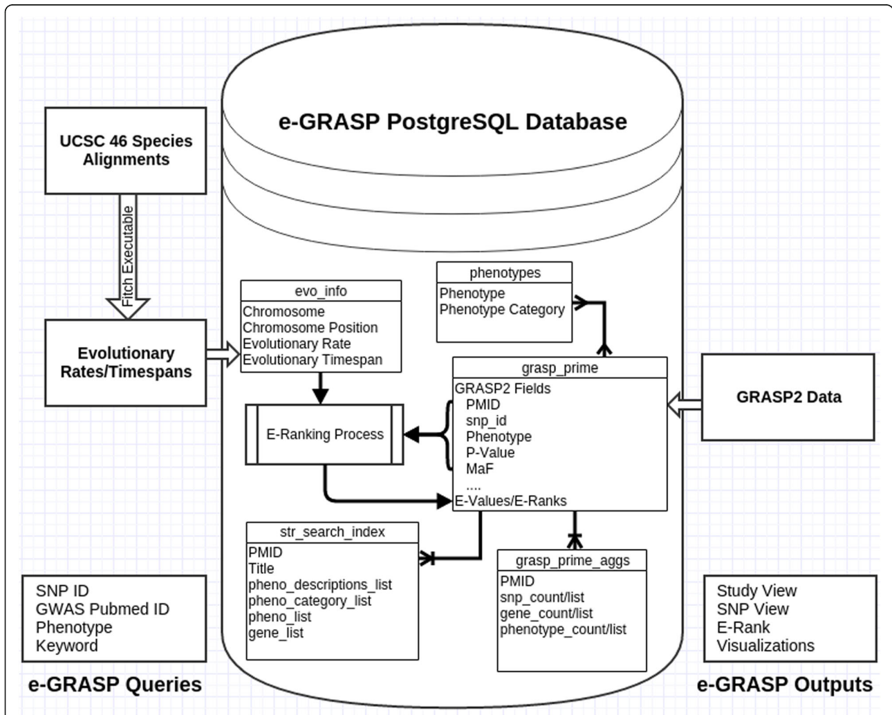
Fig. 1 e-GRASP data flow and framework. e-GRASP includes external information from the GRASP2 database and evolutionary rates and timespans calculated from a multiple species alignment (indicated by open arrows ). Internal interactions are indicated with black arrows . Searching may occur by SNP ID ( rsid ), GWAS Pubmed ID (PMID), phenotype, or keyword
